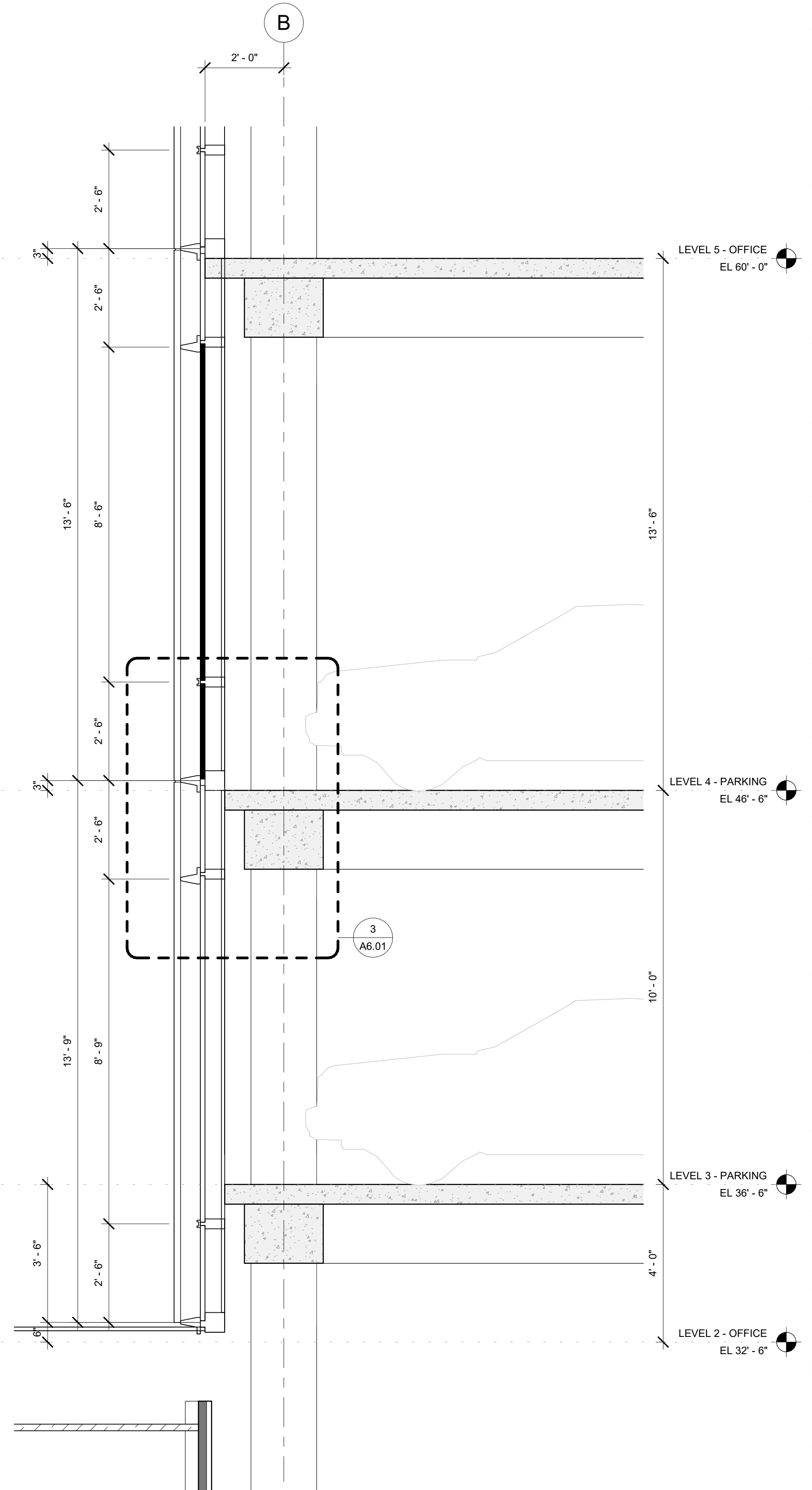
2 SECTION 1/2" = 1'-0"
