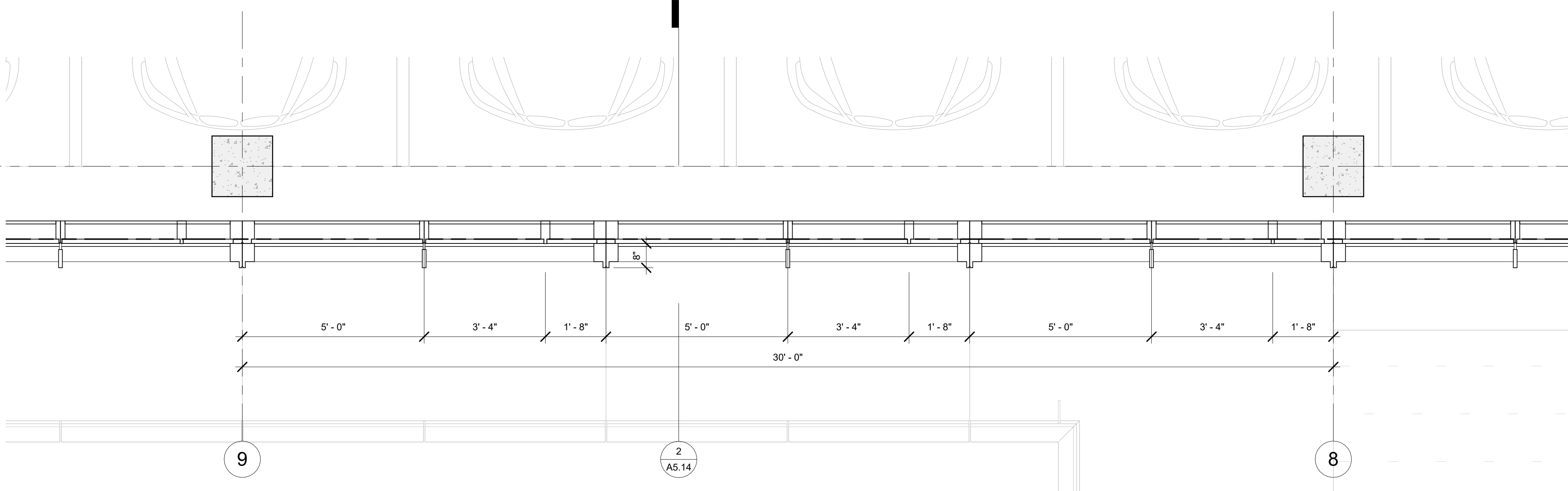
3 PLAN 1/2" = 1'-0"
