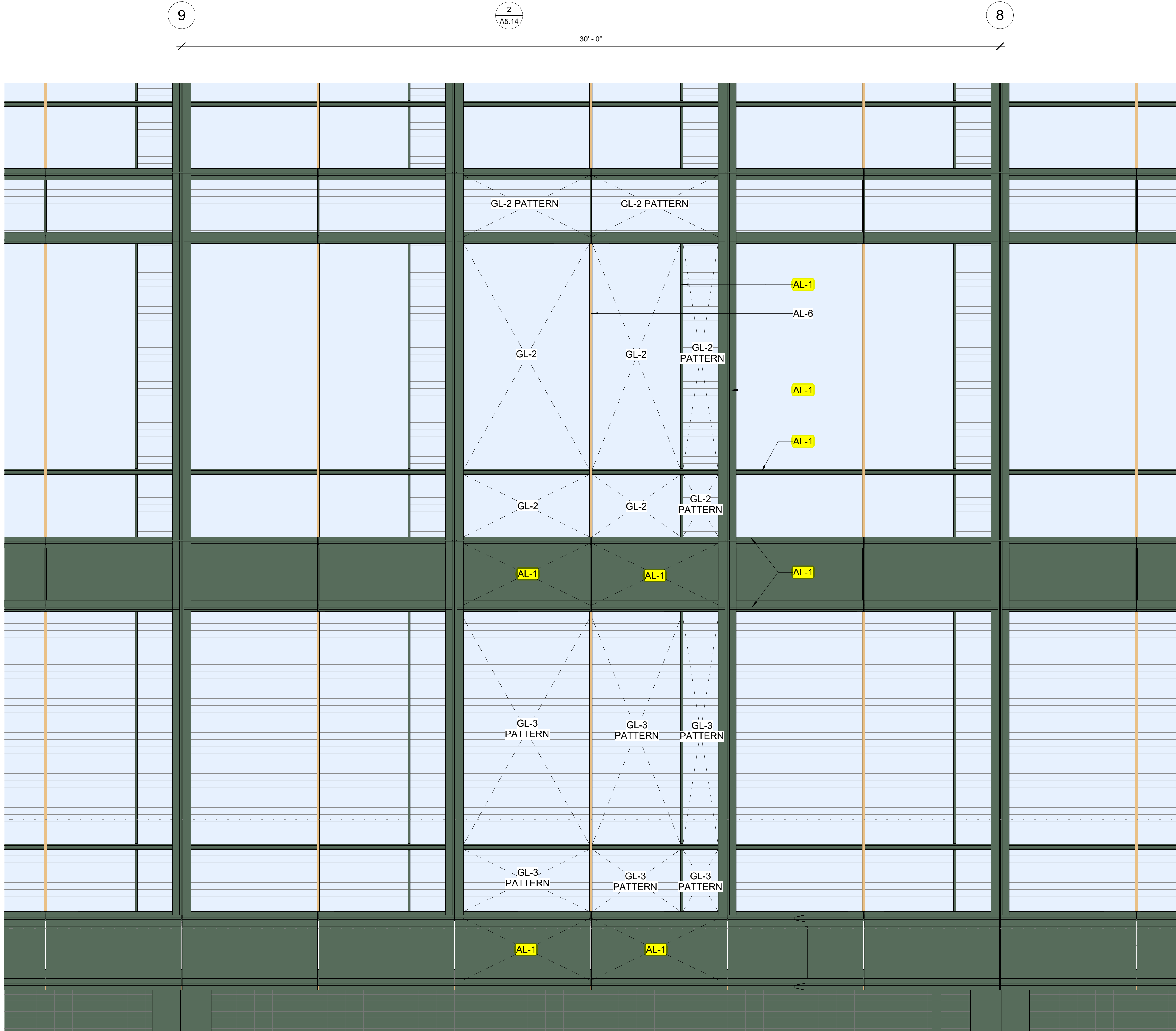
1 ELEVATION 1/2" = 1'-0"
